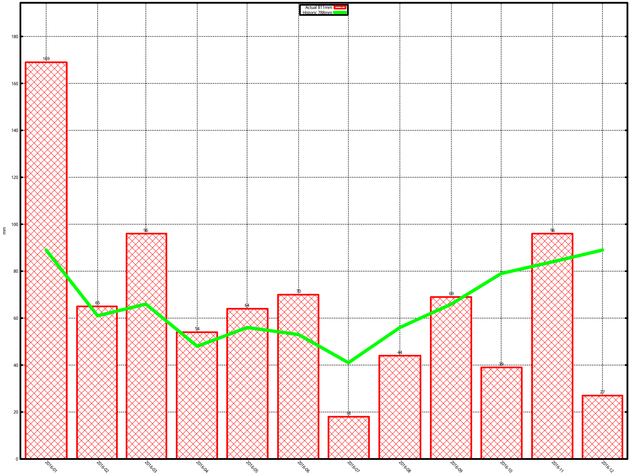
2016 Rainfall
